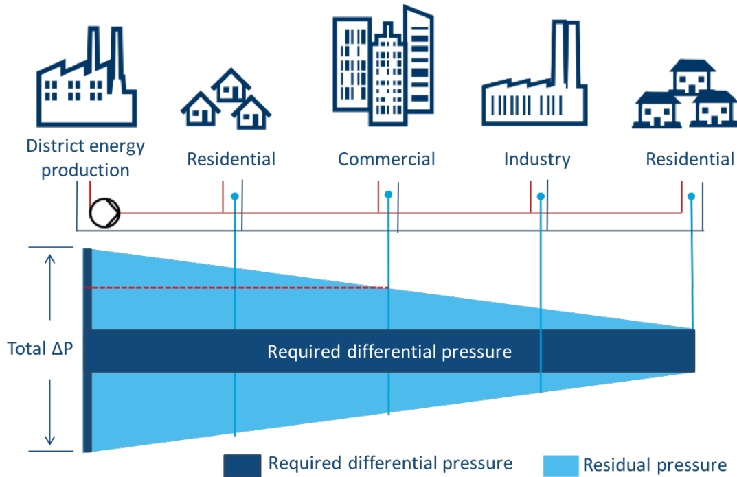
Fig 3: A lower forward pressure requires more flow (and pressure) to deliver the same the energy in the system: \Phi = Q * \Delta t
