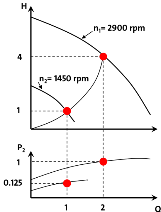
Fig 2: Consequences of increasing the pressure from factor 1 to factor 4, in line with the affinity laws
