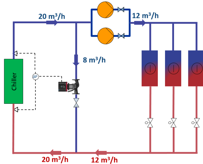
Variable primary flow system with bypass pump
